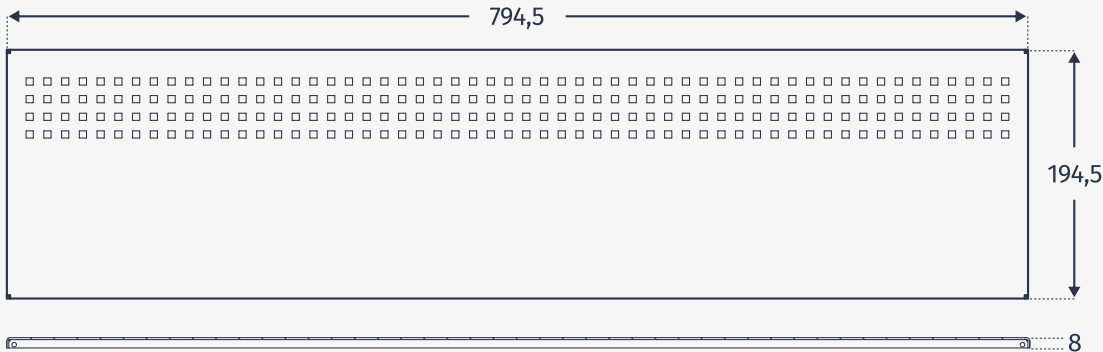
Rist | Grate
