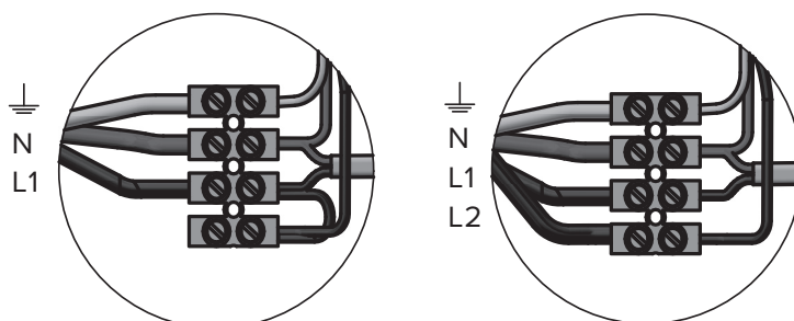
3 wire connection - 1 phase
